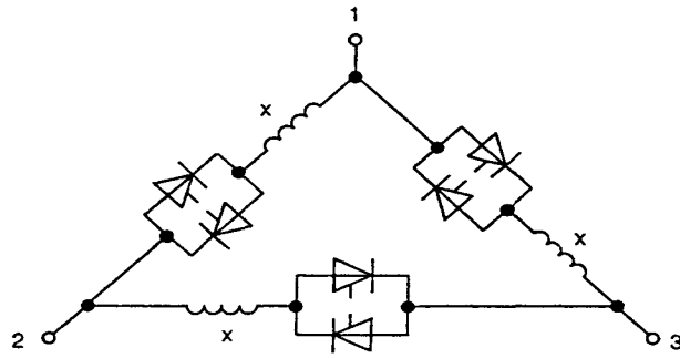
Figure 2a – Motor in delta – Thyristors in series with a winding
