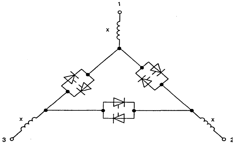
Figure 2b – Motor in star – Thyristors in delta
