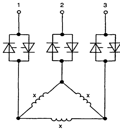
Figure 2c – Motor in delta – Thyristors connected between winding and supply
