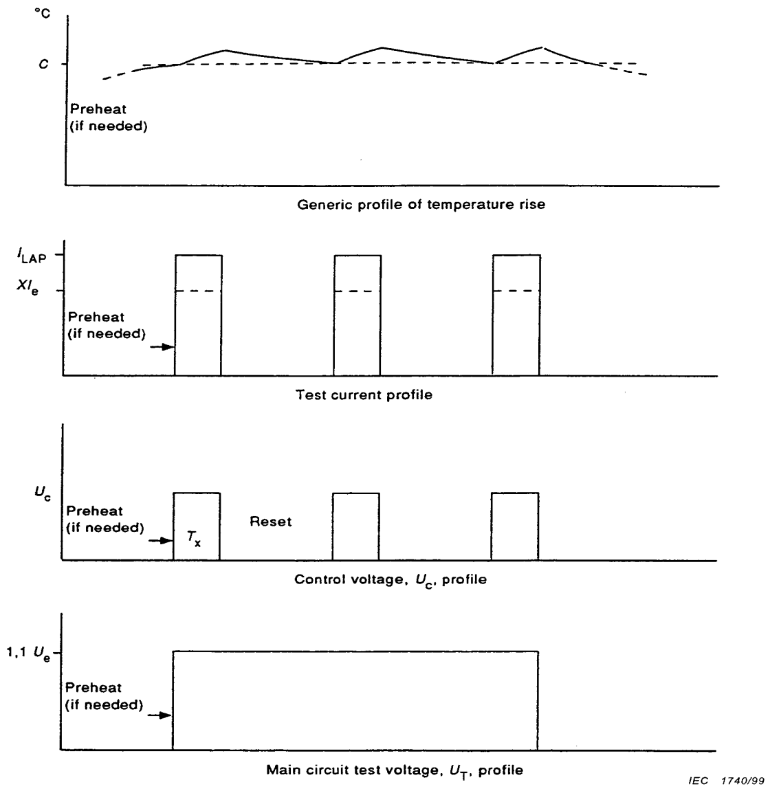
Figure F.2 – Overload capability test profile
