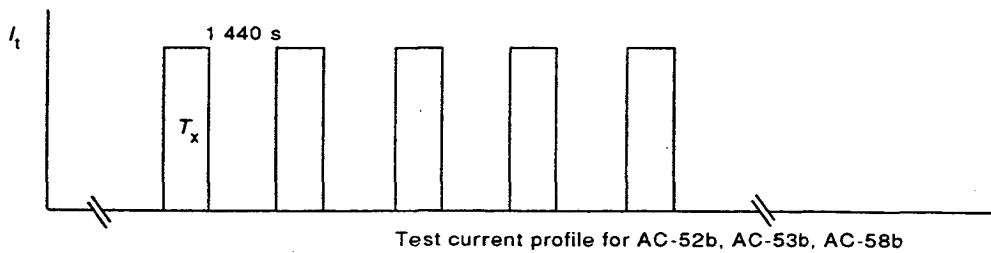
Figure F.1 – Thermal stability test profile
