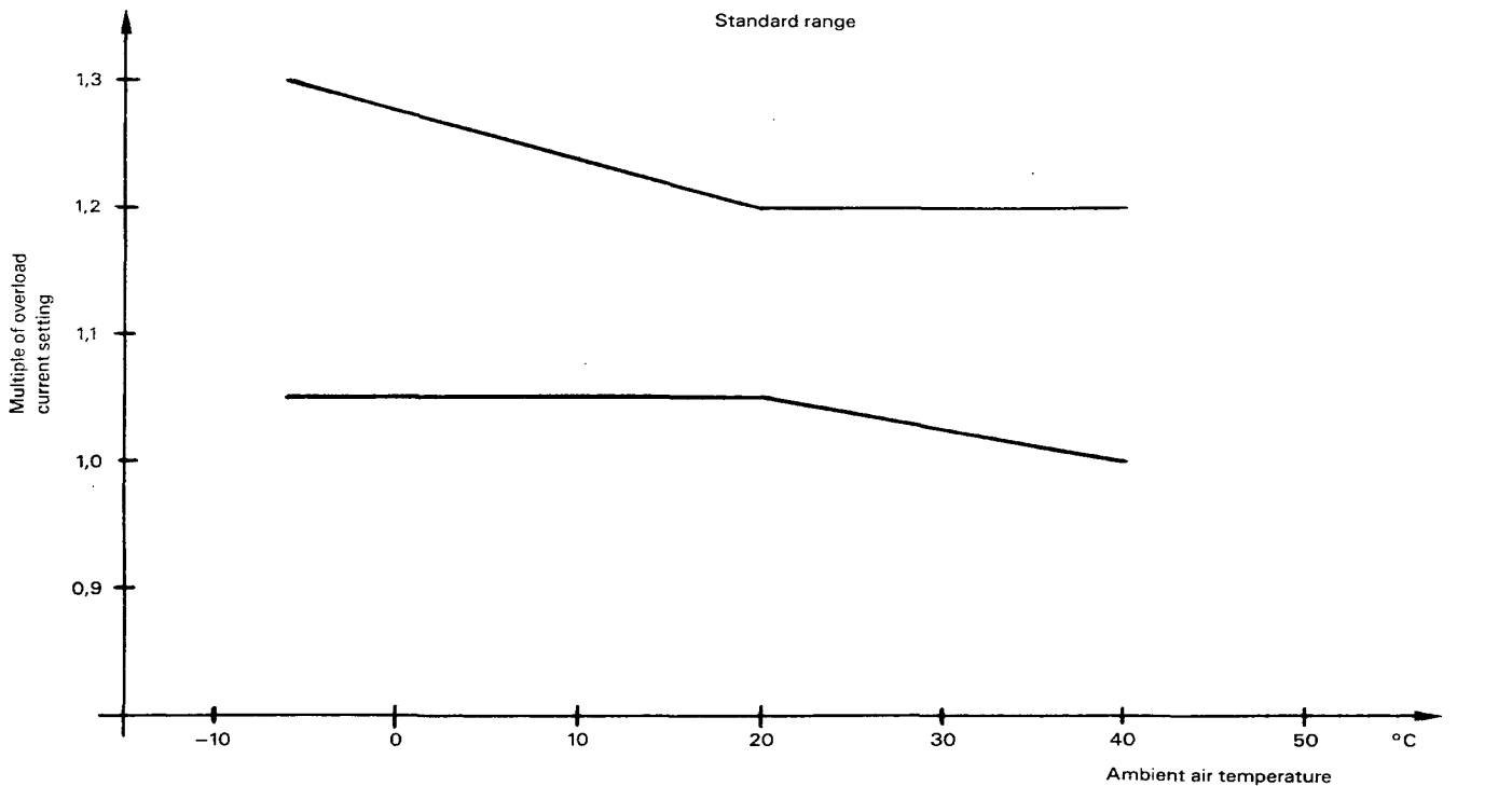
Figure B.1 - Multiple of current setting limits for ambient air temperature compensated time-delay overload relays
