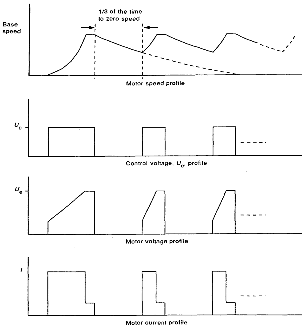
Figure F.3 – Blocking and commutating capability test profile
